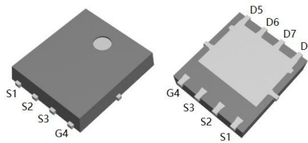
DFN5x6
